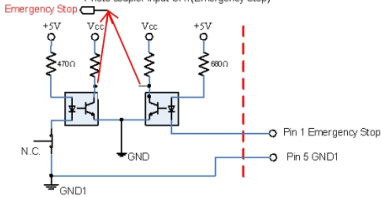
Photo coupler input CKT(Emergency Stop)
