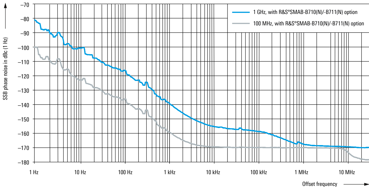
Measured SSB phase noise of the 100 MHz and 1 GHz reference outputs (R&S®SMAB-K703 option) with the R&S®SMAB-B710(N) and the R&S®SMAB-B711(N) options
