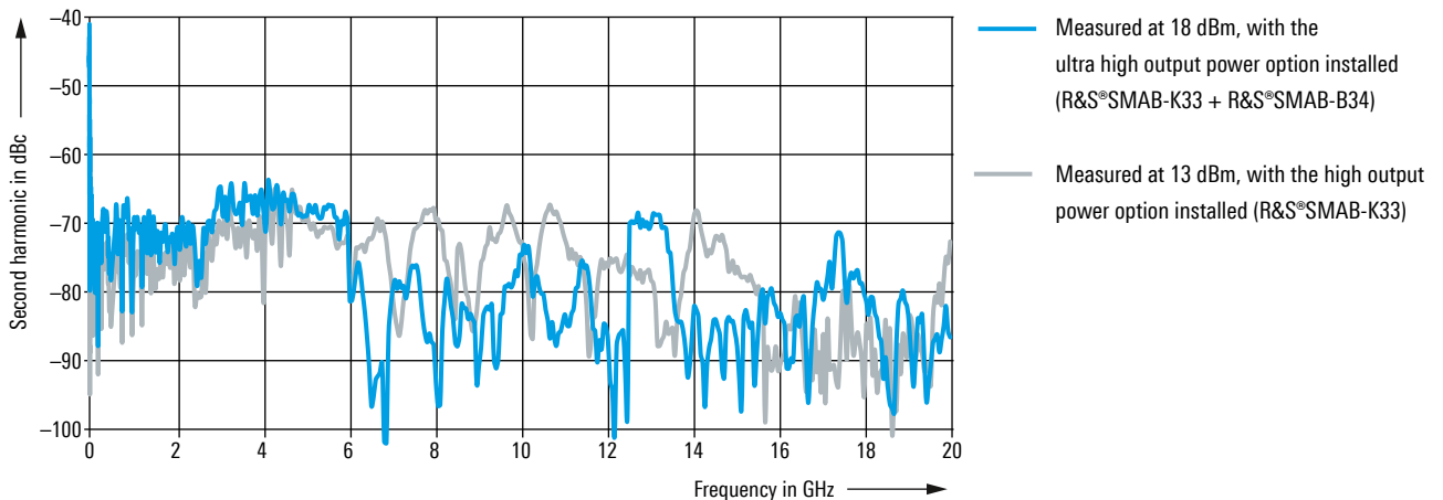
Measured harmonic performance of 20 GHz instrument
