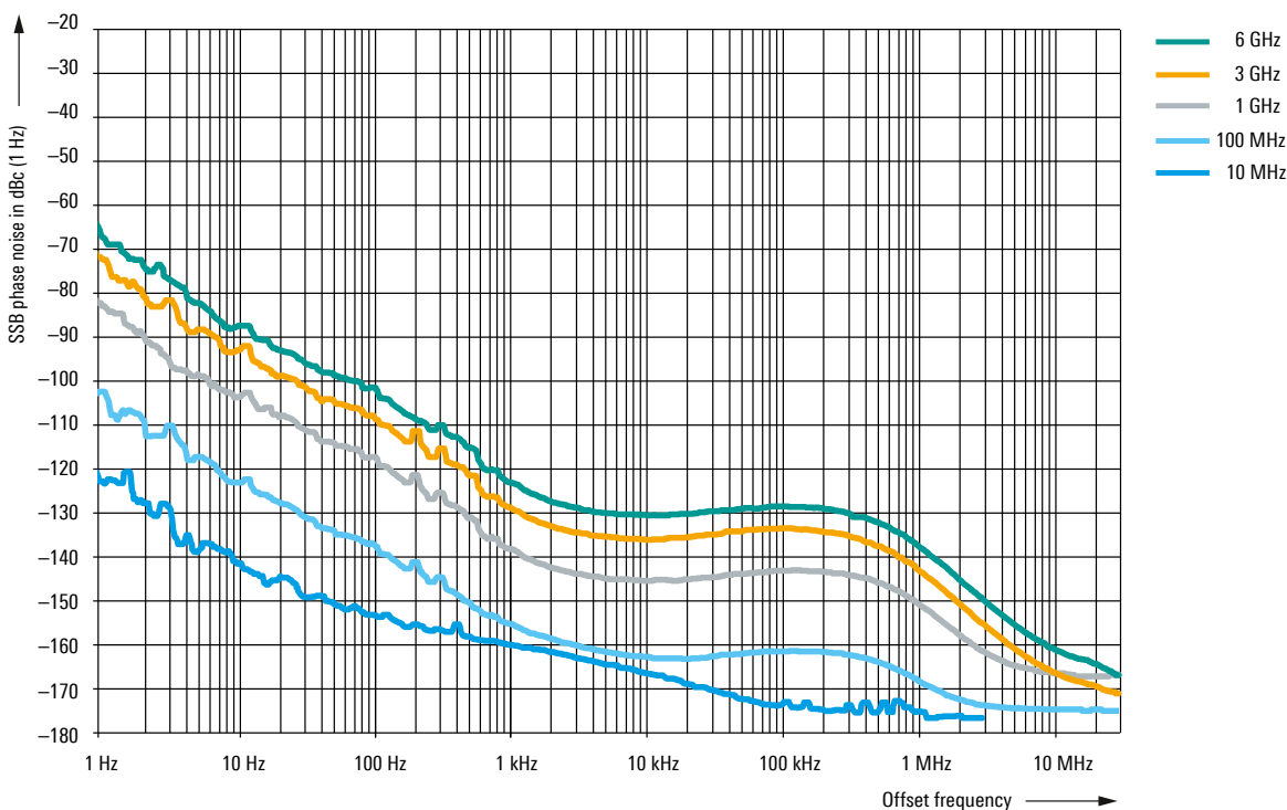
Measured SSB phase noise performance of clock synthesizer output signal with the R&S®SMAB-B29, R&S®SMAB-B711(N) and R&S®SMAB-K722 options
