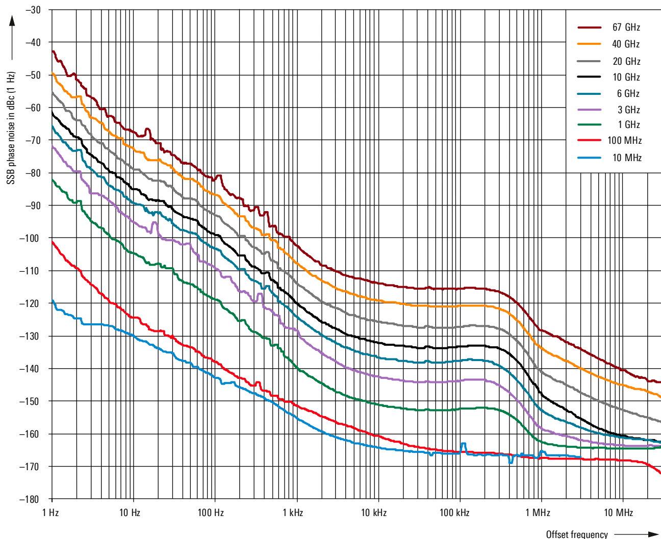
Measured SSB phase noise performance of R&S®SMA100B with R&S®SMAB-B711(N) option
