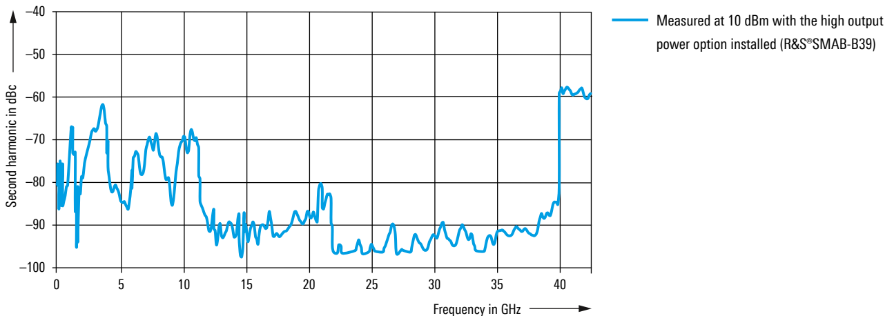
Measured harmonic performance of 67 GHz instrument
