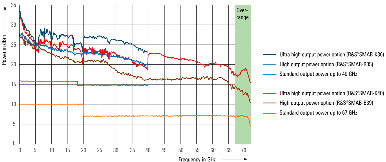
Measured maximum available output power for the 40 GHz and the 67 GHz instrument for the base unit (standard output power), with the high output power option, and with the ultra high output power option (the high output power option is a prerequisite for the ultra high output power option)
