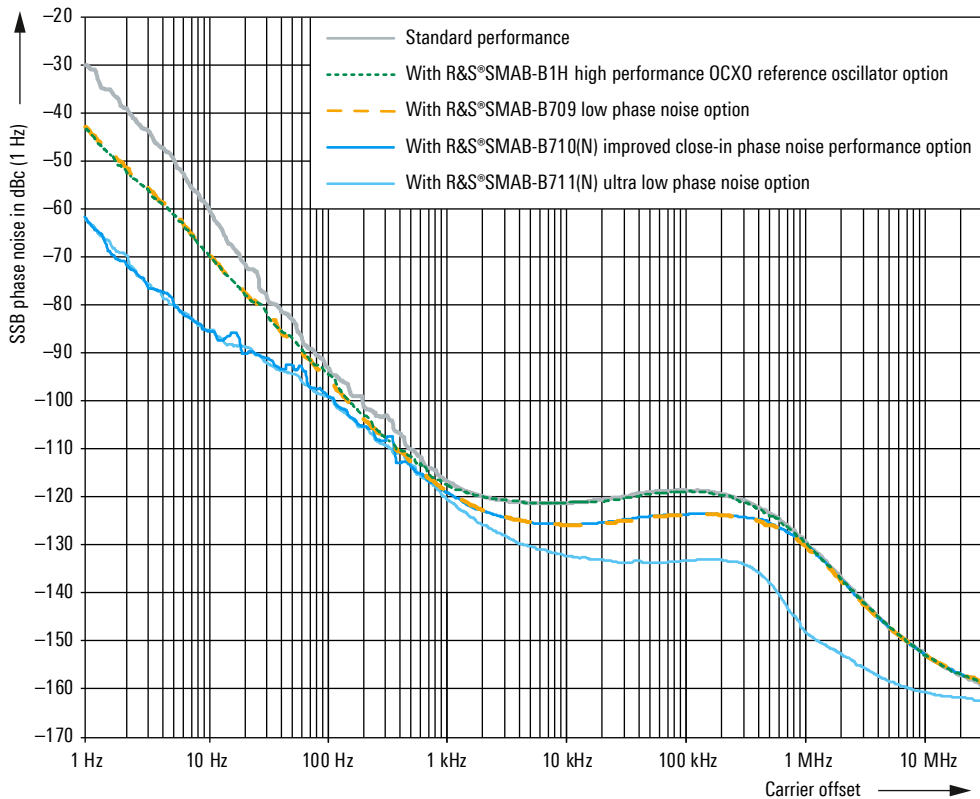
Measured SSB phase noise performance of R&S®SMA100B at 10 GHz
