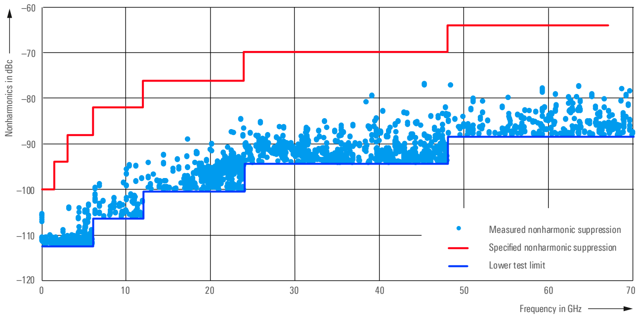
Measured nonharmonic values ( f_{\text{offset}} \geq 10 kHz) with R&S®SMAB-B711(N) option
