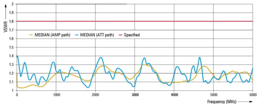
VSWR vs. frequency (with R&S®SMBB-B32 option)
