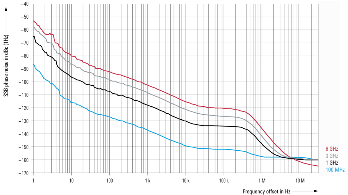
Measured SSB phase noise with R&S ® SMBB-B1H option.
